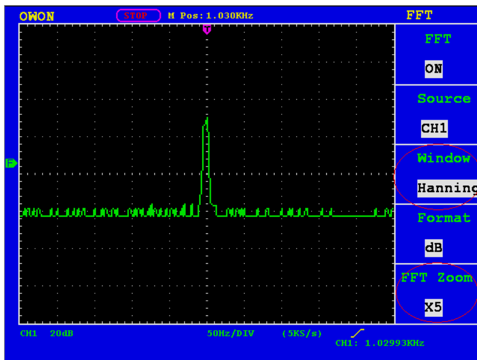
Fig.24 Hanning window
