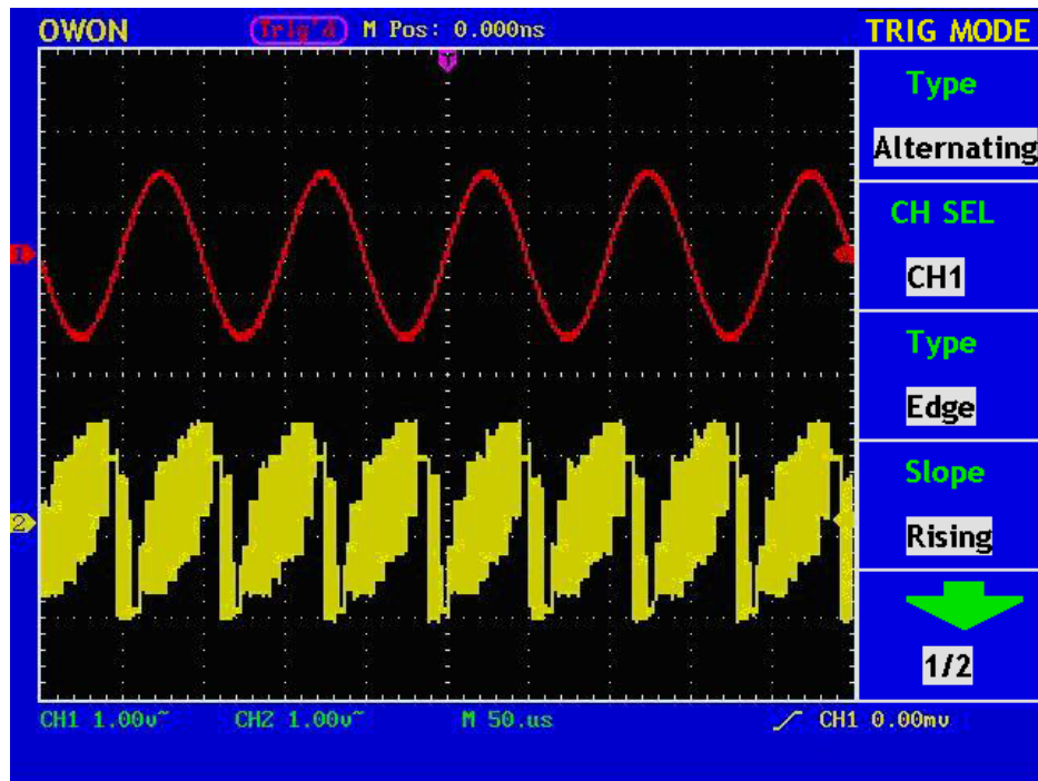
Fig.42 Alterate trigger waveform
