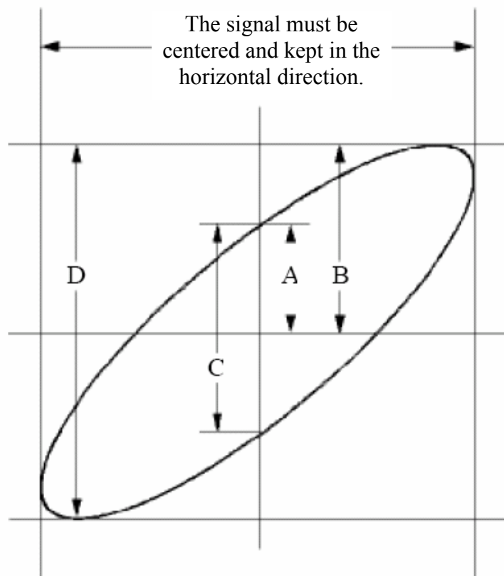
Fig.70 Lissajous Graph
