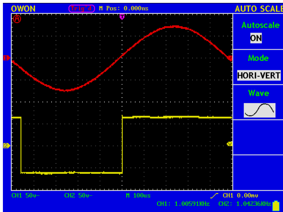
Fig.63: Autoscale Horizontal- Vertical mono-period waveform
