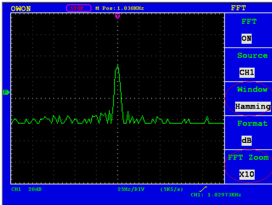
Fig.22 Hamming window
